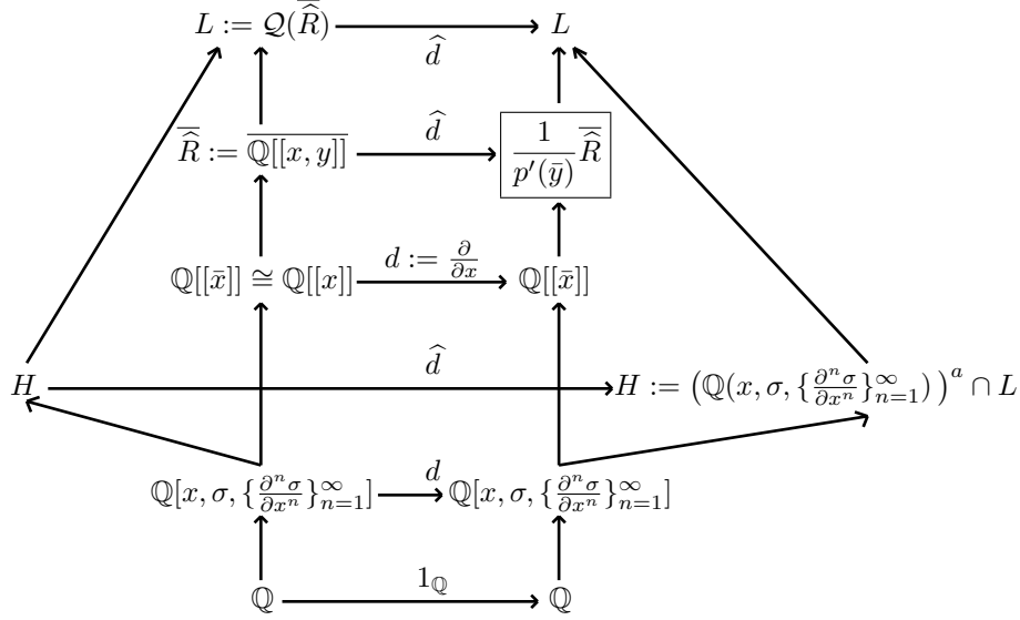
Picture \boxed{7.6.5.4} \boxed{12.19.1} . The image of subrings of L via the extension \widehat{d} of d := \frac{\partial}{\partial x} .
